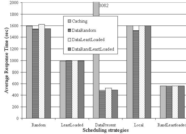
Figure 1.2. Average response time for different combinations of scheduling and replication strategies.
