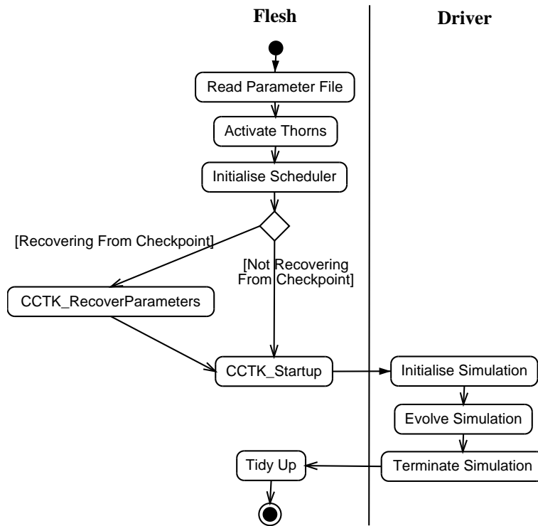
Fig. 1. The main flow of control in the Cactus Framework. The flesh initialises the code, then hands control to the driver thorn (see section 10). The actions in the driver swimlane are detailed in figures 2, 3, and 4.
