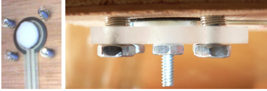
Figure 13. Sandwich elements shown with motorized fader removed (left: bottom view also with acrylic removed, right: side view with acrylic)
