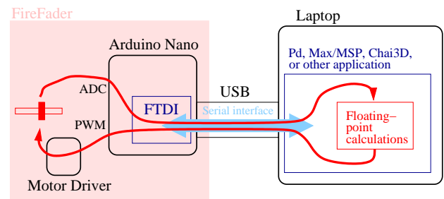
Figure 5. Signal flow for the control loop
