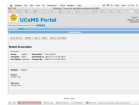
Fig. 5. Job Output
