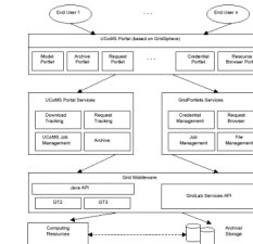
Fig. 6. UCoMS Portal Architecture
