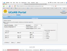
Fig. 4. User Input
