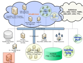
Fig. 3. Resource Grid
