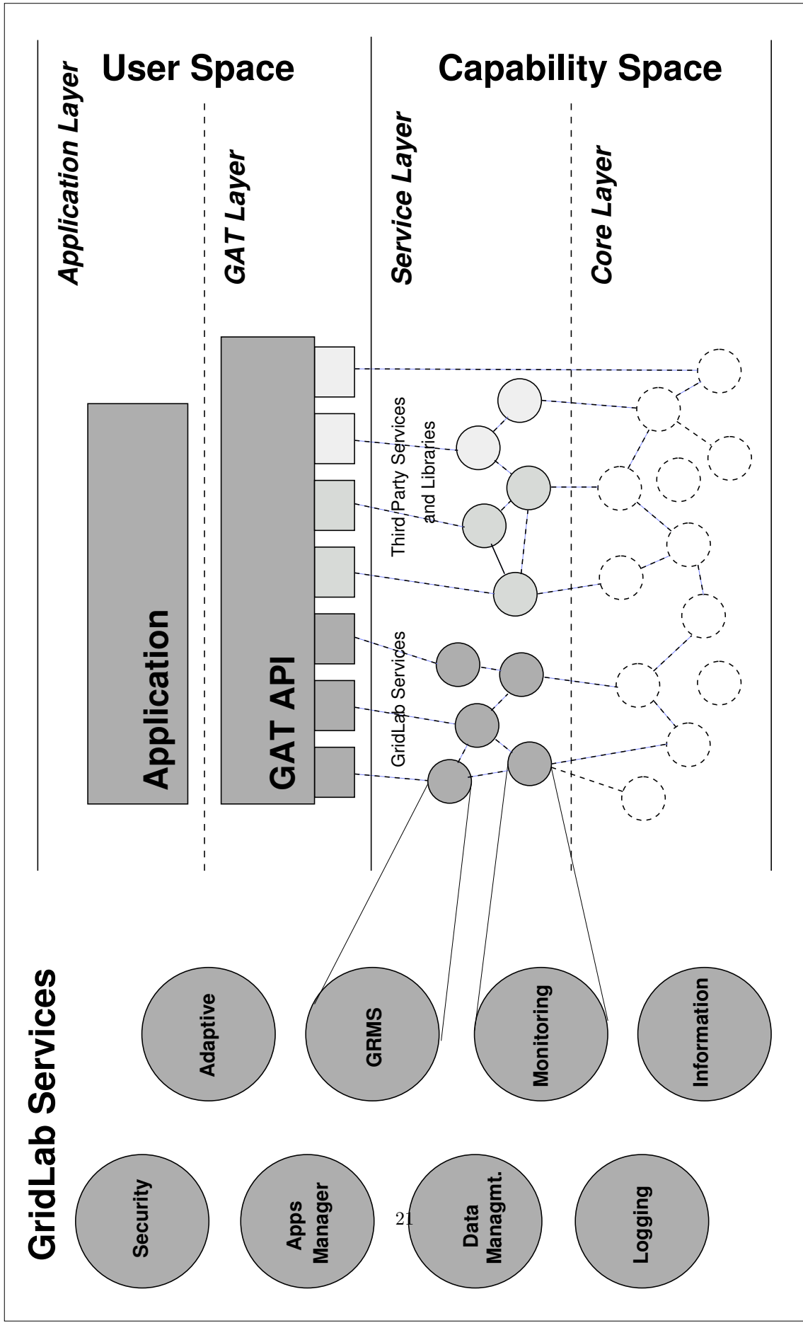
Figure 1: The General GridLab Architecture: The GAT will be designed to interact with all types
