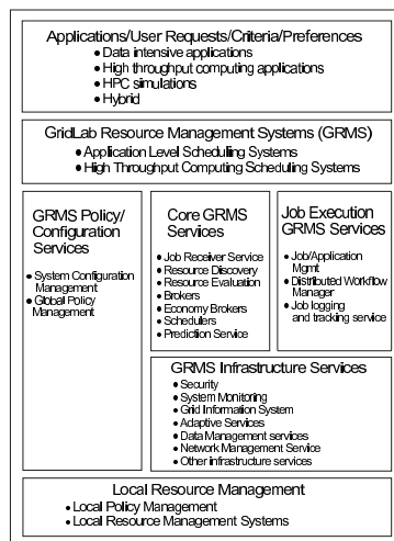
Figure 6: Reference architecture of the GridLab Resource Management System (GRMS).
